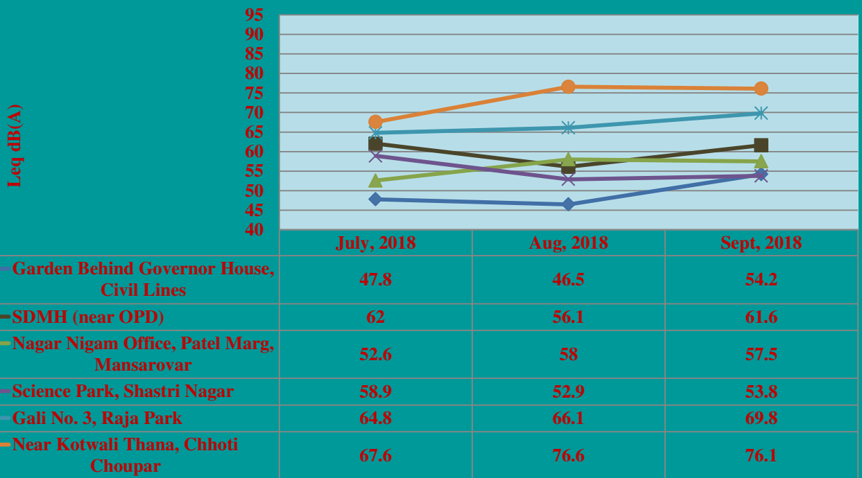
Fig. 2 Noise Level during Night time from July to September in Jaipur City
